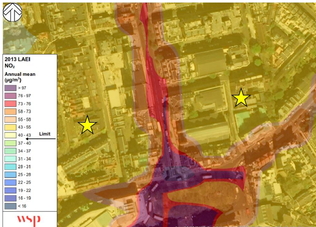
Figure 5 – Localised Air Quality modelling around Holy Trinity
