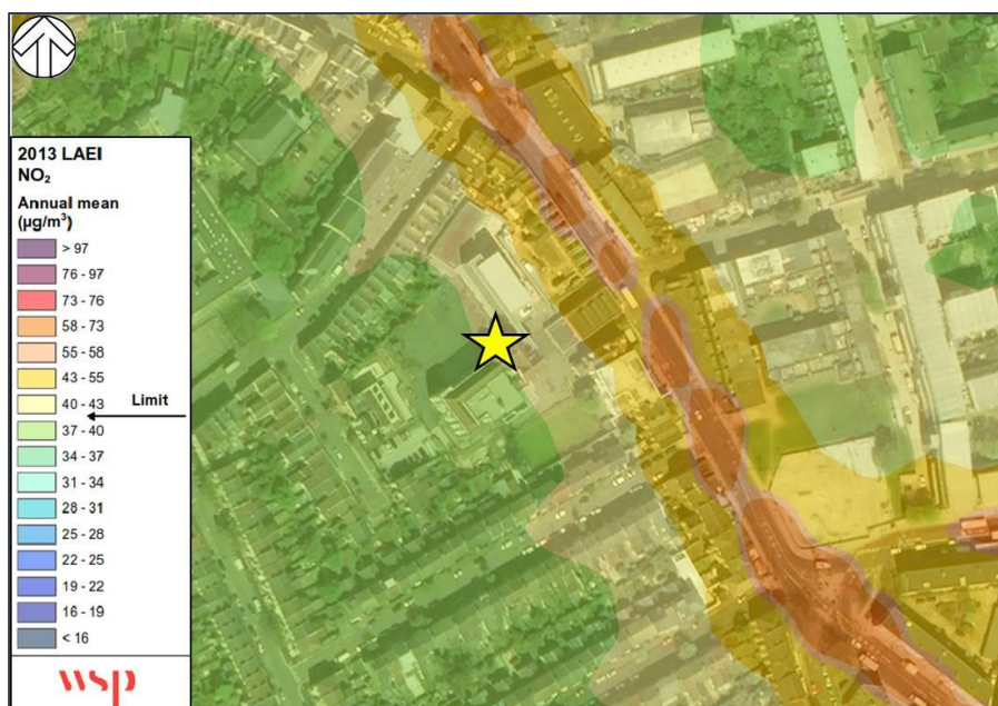
Figure 5 – Localised Air Quality modelling around Stockwell Primary School
